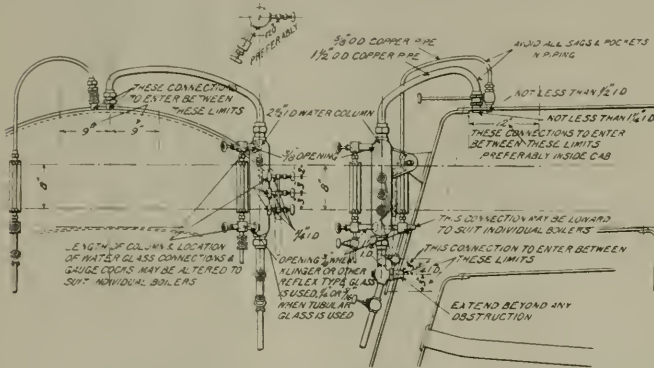
FIG. 11. RECOMMENDED PRACTICE ARRANGEMENT OF GAUGE COCKS AND WATER GLASSES.
